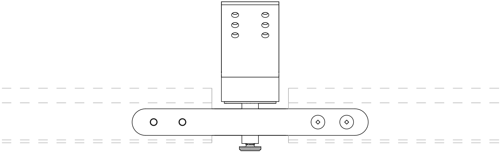
GAPLOK / TRACKLOK® ASSEMBLY | SIDE ELEVATION
