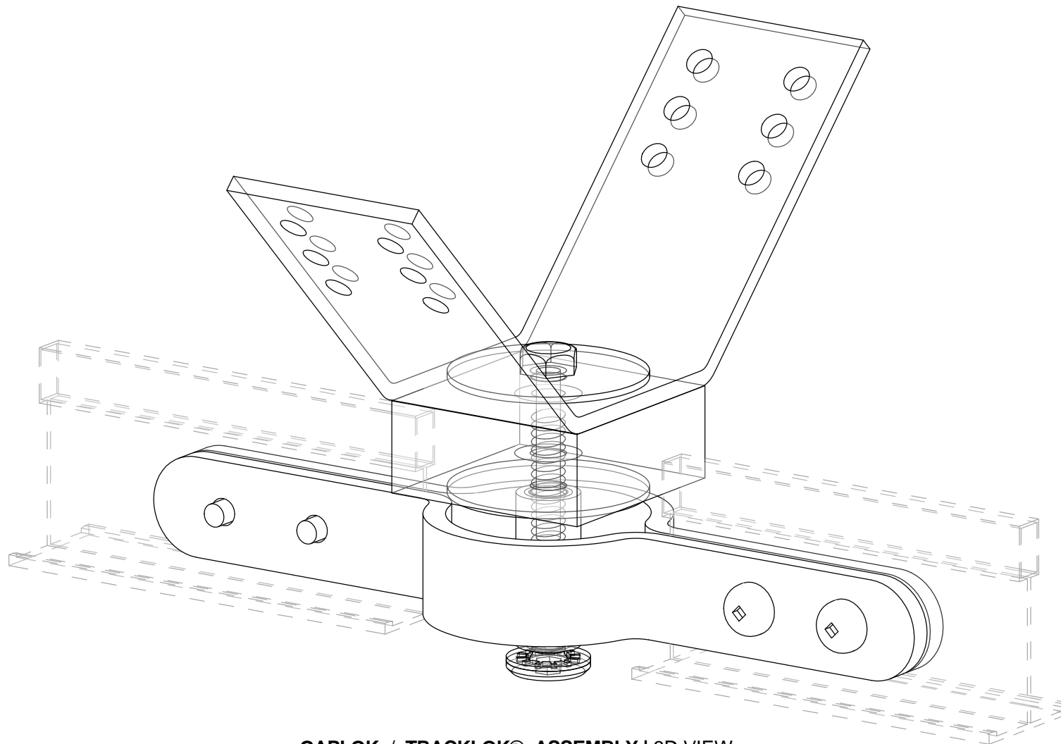
GAPLOK / TRACKLOK® ASSEMBLY | 3D VIEW
