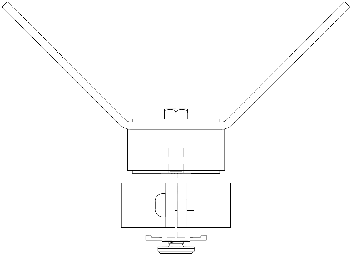
GAPLOK / TRACKLOK® ASSEMBLY | END ELEVATION
