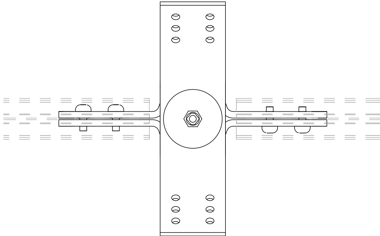
GAPLOK / TRACKLOK® | PLAN VIEW
